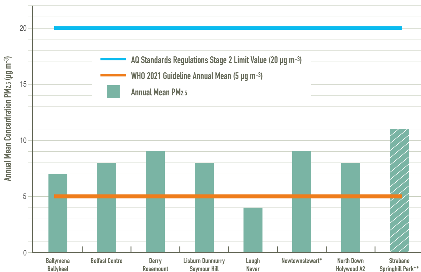
Figure 4.3: Annual Mean PM 2.5 Concentrations for 2022
