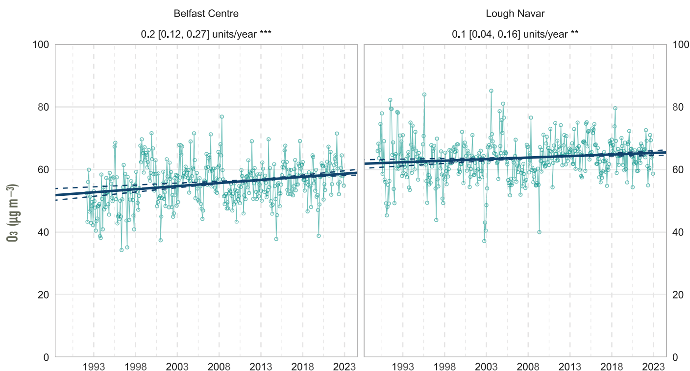
Figure 5.2: De-seasonalised trend plots for O_3 measured at Lough Navar from 1990 to 2022 and Belfast Centre from 1992 to 2022.
