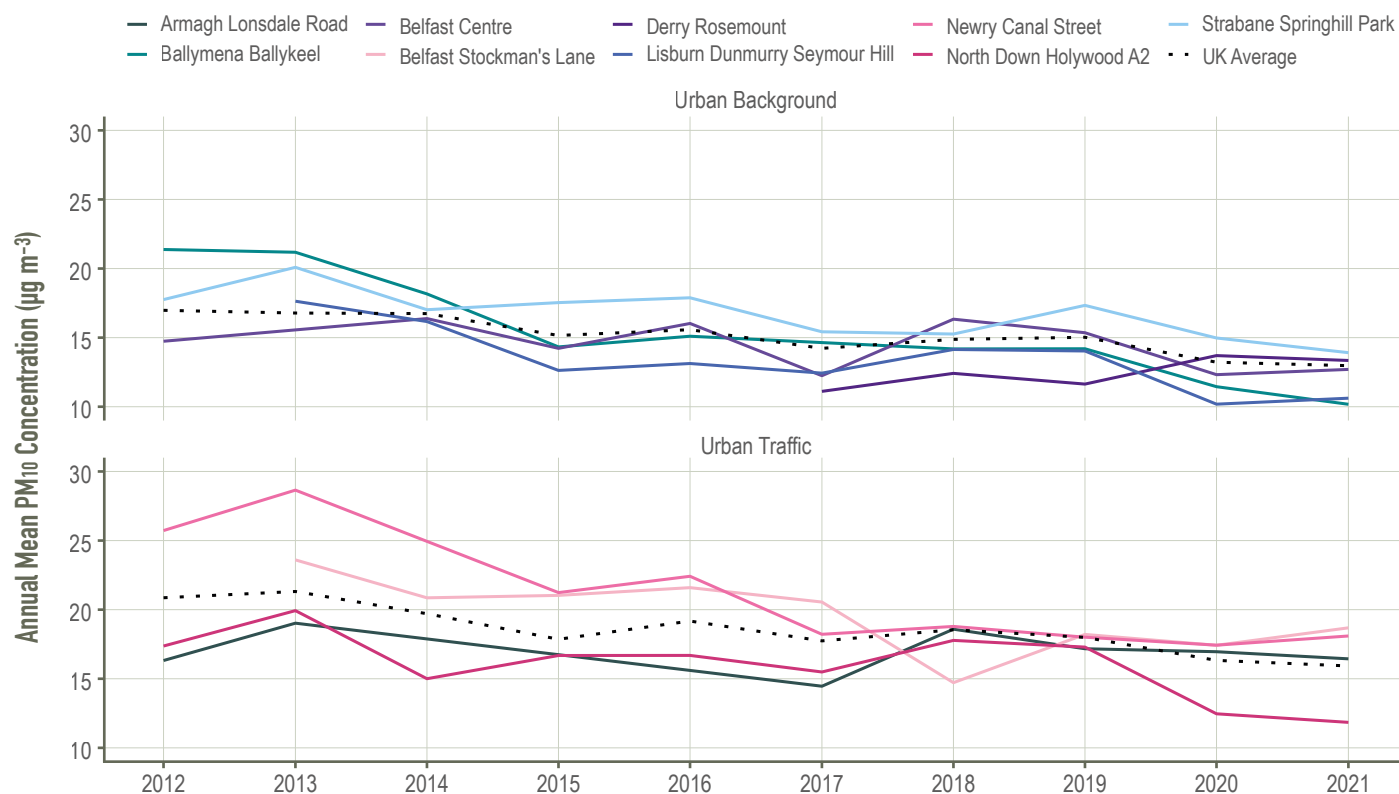
Figure 5.1: Comparison of annual mean concentrations of PM 10 at urban traffic and urban background sites (with a data capture > 75% for each year) in Northern Ireland (solid lines) to the UK average (dashed line), from 2012 to 2021
