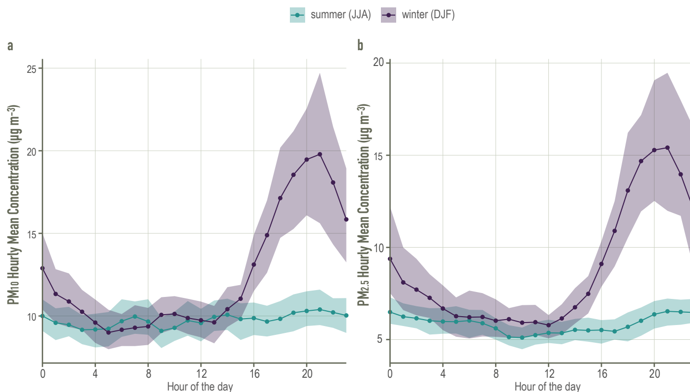
Figure 6.3: Diurnal graph of hourly averaged concentrations of a) \text{PM}_{10} and b) \text{PM}_{2.5} for winter and summer months in 2021, measured at Lisburn Dunmurry Seymour Hill. Shaded regions represent the 95 th percentile of the mean
