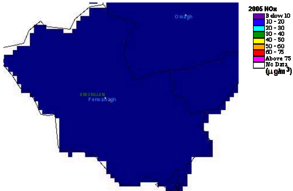
Figure 3.1. NO x background concentrations for 2005( \mu\text{g}/\text{m}^3 )
